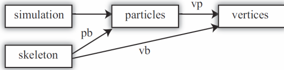
Figure 2: The upper row shows the basic OP flow: the particles are driven by the simulation while the vertex positions are computed from the particle positions via skinning. With a rigged mesh the particles can either be driven by simulation or the skeleton, while the vertices can be skinned either to the particles or directly to the skeleton.
