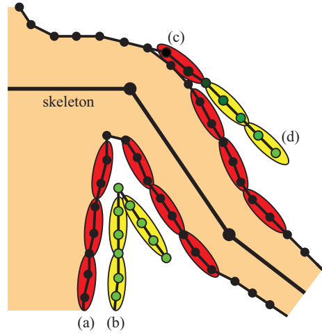
Figure 3: 2D cross section through a simulation of a shirt on a character. The inputs are a visual mesh for the skin (a) and a visual mesh for the shirt (b) with skinning information. Oriented particles are placed on the visual meshes. The yellow particles are simulated and the red particles animated, following the skeleton. Animated particles are used to attach the simulation mesh (c) or as collision primitives (all others). The vertices of the visual meshes are marked to be skinned to either the skeleton (black) or the particles (green) with smooth transitions as between vertices (c) and (d).
