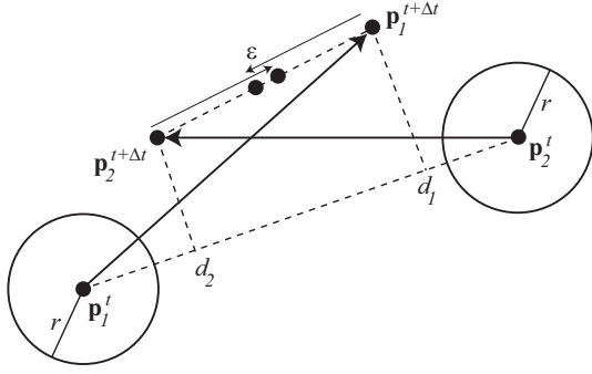
Figure 5: Approximate continuous collision handling for two spherical particles with radius r . If, during the time step \Delta t , the distance between two particles becomes smaller than 2r , we check whether their projected positions on the line \mathbf{p}_1^t - \mathbf{p}_2^t got inverted. If so, we flip their positions along the line \mathbf{p}_1^{t+\Delta t} - \mathbf{p}_2^{t+\Delta t} to conserve momentum.
