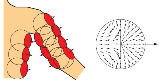
Figure 6: Surface particles have their first axis aligned with the mesh normals. For collision, they are replaced by a sphere tangent to the ellipsoid at the extremal point of this axis for robust collision handling. The knowledge of the outward direction can also be used to modify the direction in which colliding particles are projected out of the sphere to prevent entanglements.
