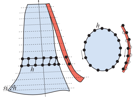
Figure 7: Vertical and horizontal cross sections of a coat and cape. Particles (black dots) are placed on the cut lines of the meshes with horizontal planes. A particle is only created if there are no close particles already placed on the mesh. If desired, edges (thick black lines) are created between subsequent particles on a cut line and between particles on neighboring horizontal planes.
